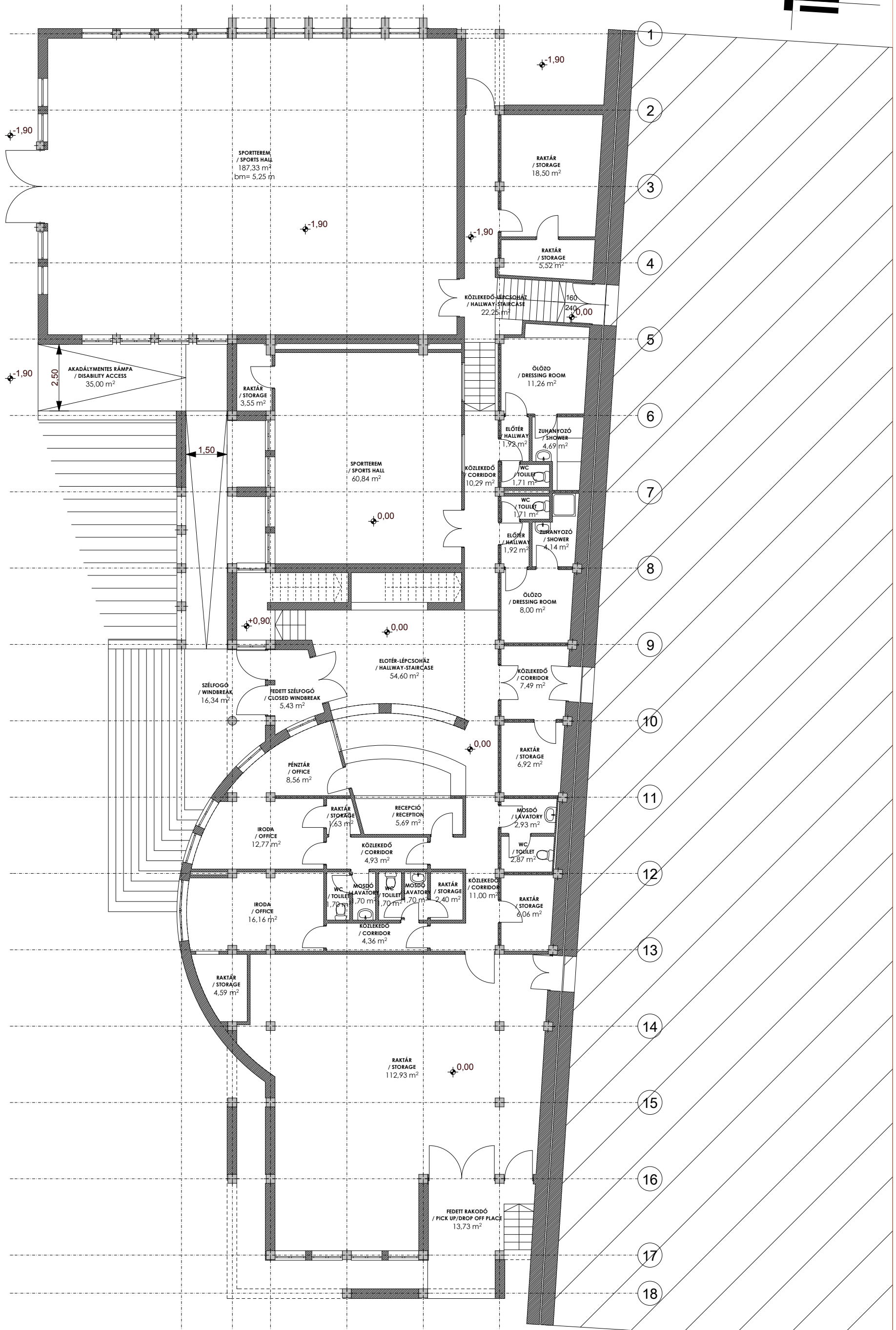
FÖLDSZINT ALAPRAJZA / WEST WING OF BUILDING GROUND FLOOR
